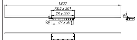
Duschrinne CeraWall Connect messing matt
