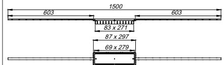
Duschrinne CeraFloor Connect schwarz matt
